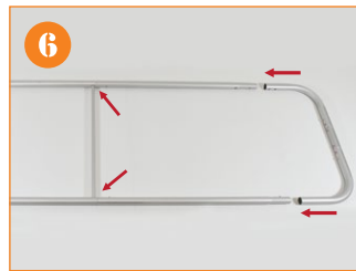
6. Insert the middle pole between two long tubes, and finish the panel with the other tubes marked E, F, G, H.
